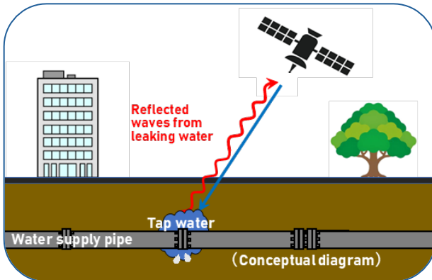
Leakage detection system for water supply pipes using satellite imagery
